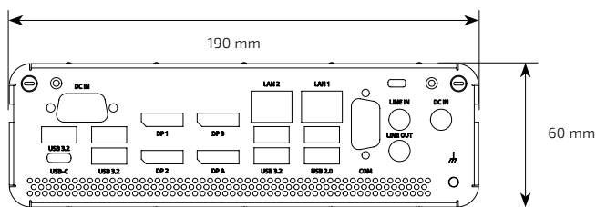
// Rear Panel
